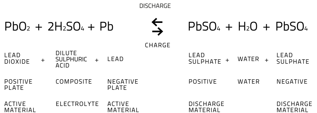
Figure 2.1. The main electrochemical reaction during charge / discharge.
