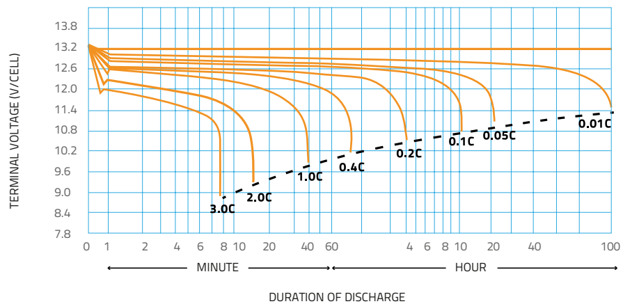
Figure 3.2 Generic curve of different discharge rates of a Lead Crystal® battery at 25°C. For discharge values of a specific battery model we revert to the constant current discharge tables in the datasheets.
